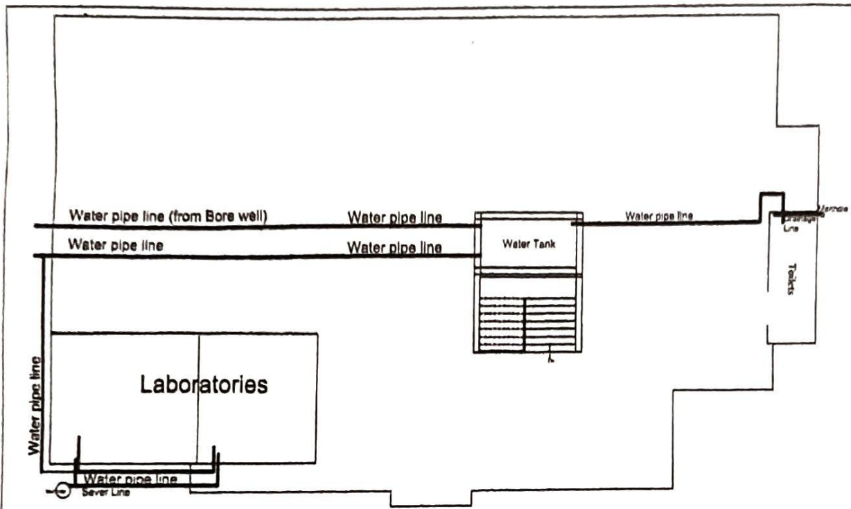
Plan of Block-E, Water Pipe Line, Sever Pipe Line and Drainage Pipe Line
